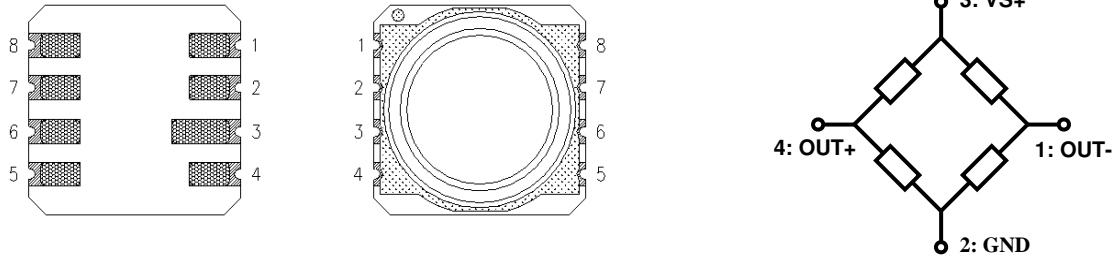
VERSION WITH CERAMIC CARRIER AND METAL CAP
