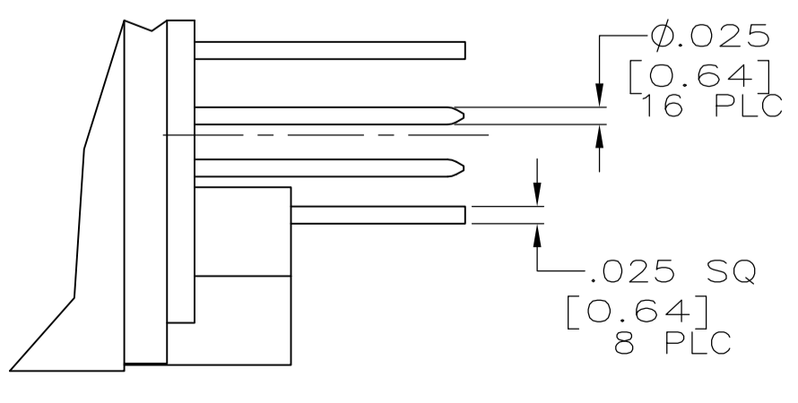
DETAIL T SCALE 4:1 SIZE 8 QUADRAX ONLY
