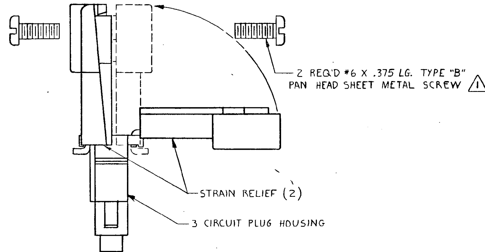
ASSEMBLY DETAILS
