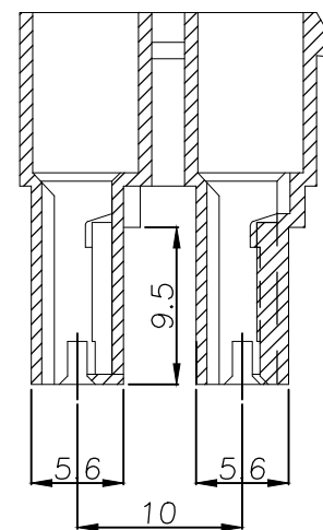
SECT. A-A
