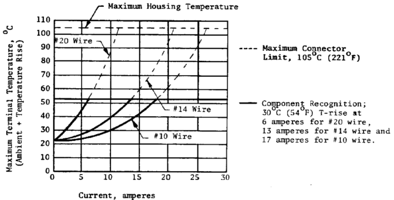
Figure 2 Terminal Temperature vs. Current/Circuit, Phosphor Bronze Contacts, 9 Circuit Free Hanging Housing
