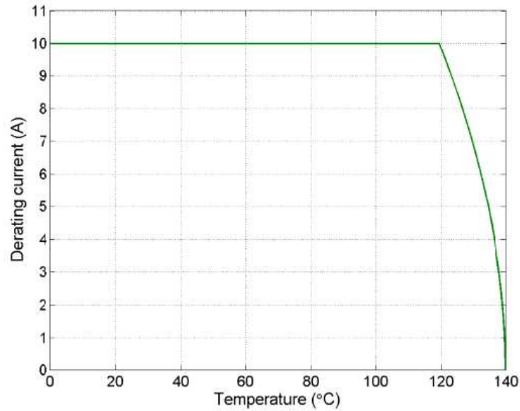
Appendix 4: 14 AWG Temperature Rise – High Temp Terminals 1971781-2 and 1971782-2 in 3x5 GWT Cap and Plug Housings
