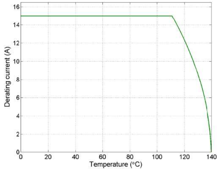
Appendix 5: 14 AWG Temperature Rise – High Temp Terminals 1971781-2 and 1971782-2 in 1x3 GWT Cap and Plug Housings
