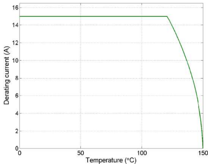
Appendix 3: 14 AWG Temperature Rise – High Temp Terminals 1971781-2 and 1971782-2 in 1x3 High Temp (150°C) Cap and Plug Housings
