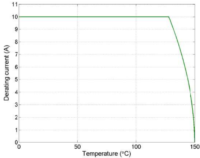
Appendix 2: 14 AWG Temperature Rise – High Temp Terminals 1971781-2 and 1971782-2 in 3x5 High Temp (150°C) Cap and Plug Housings
