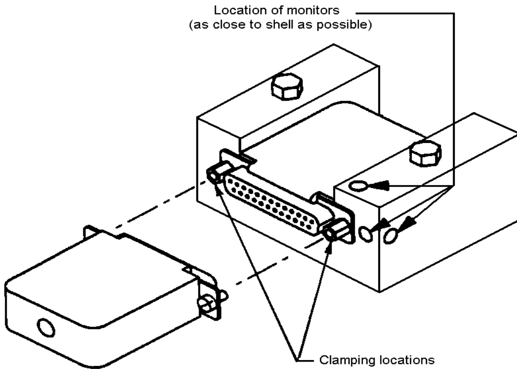
Figure 4 Vibration and Physical Shock Mounting and Clamping Locations
