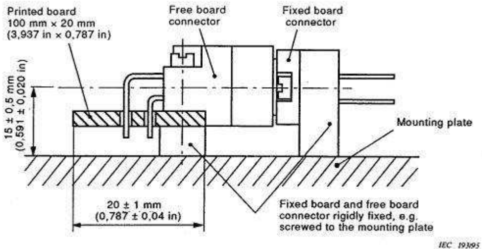
Fig.8 Arrange for connectors without cable/wires
