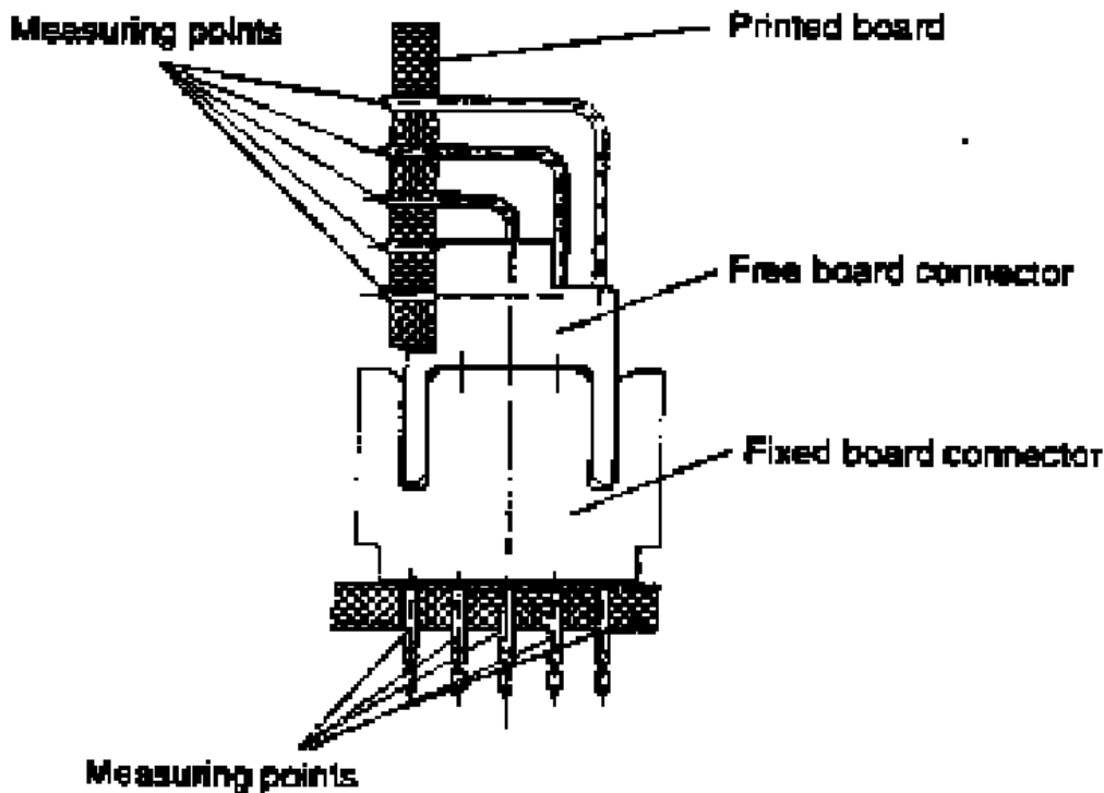
Fig. 6 Typical Terminal Resistance Measurement points
