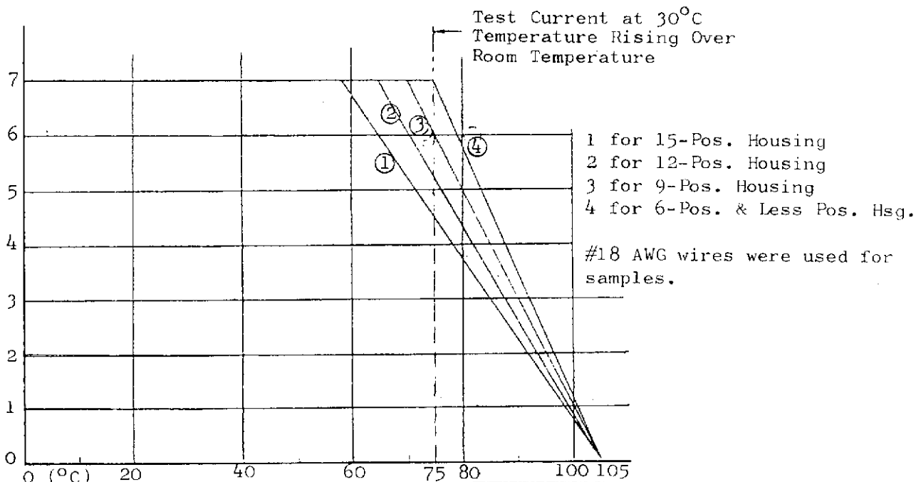
Fig. 1 Ambient Temperature Vs. Loaded Current
