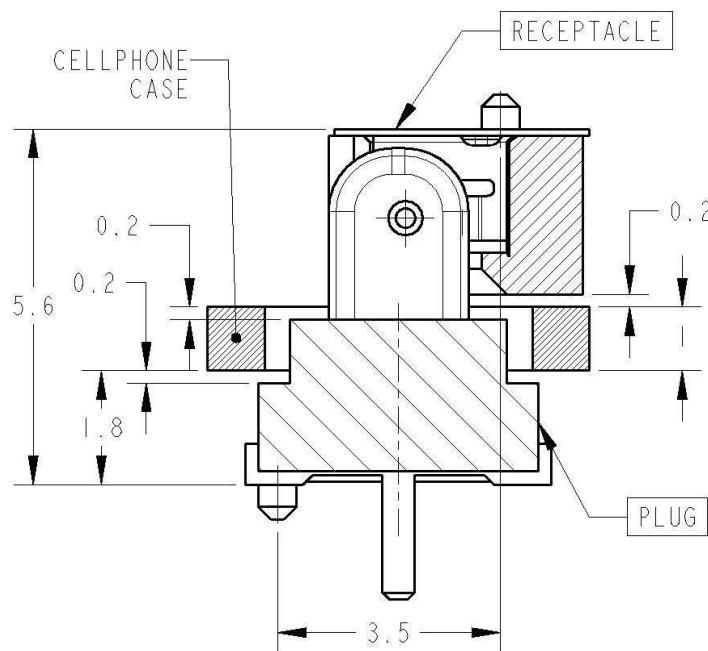
Fig.2 MATING CONNECTOR
