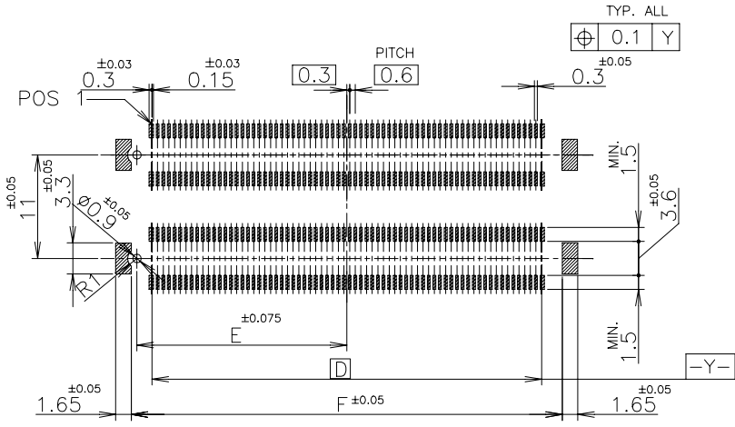
REFERENCE P.C. BOARD LAYOUT
