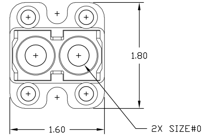
REAR VIEW
