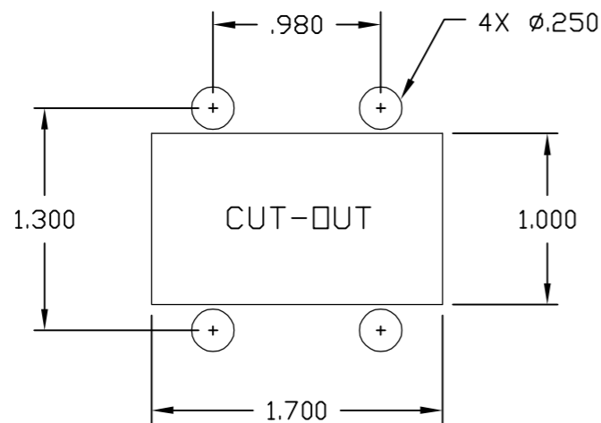
PANEL MOUNT
