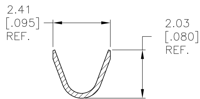
SECTION F-F INSULATION RANGE: \phi 1.75 [.069] MAX.
