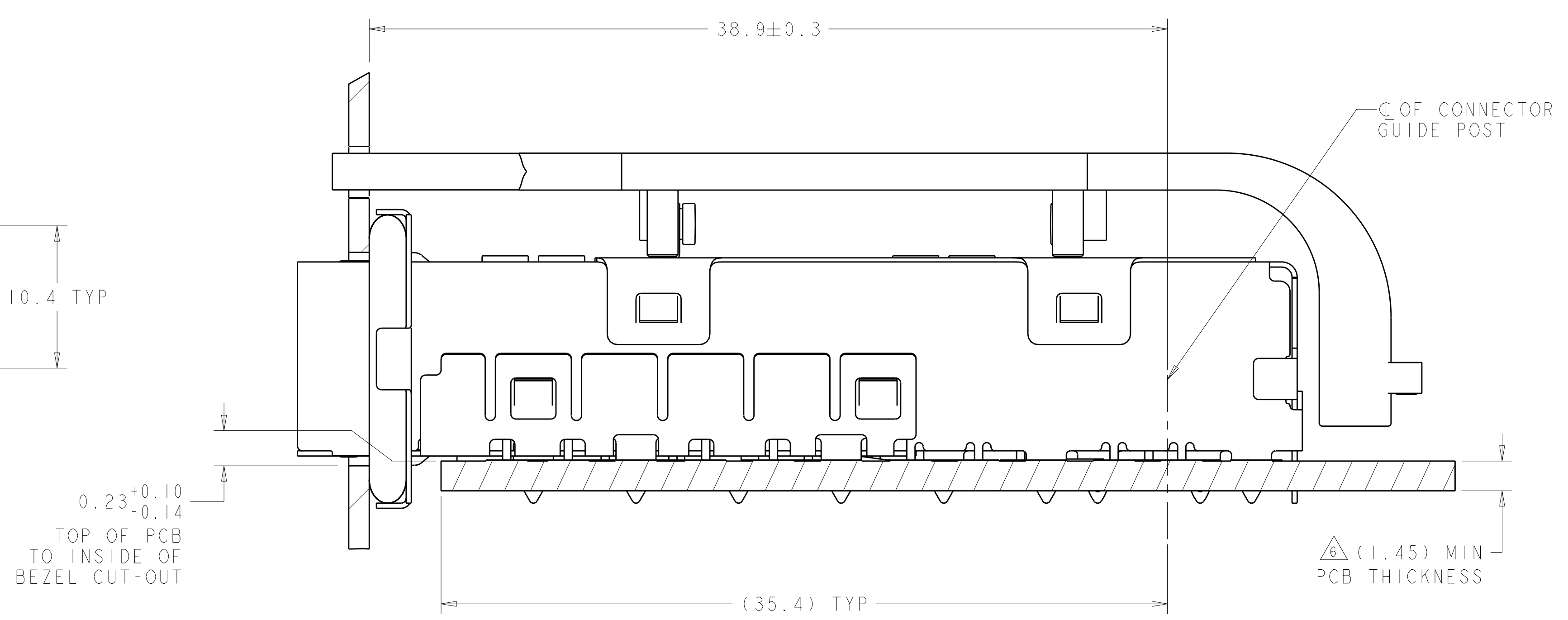
2057112-1 MOUNTED ON PCB SHOWN THRU RECOMMENDED BEZEL
