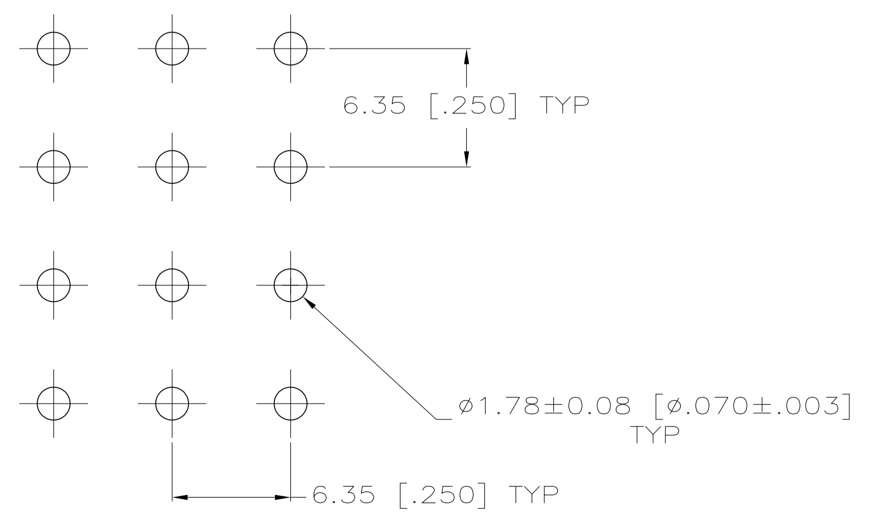
RECOMMENDED LAYOUT FOR 1.58 [.062] THICK PC BOARD
