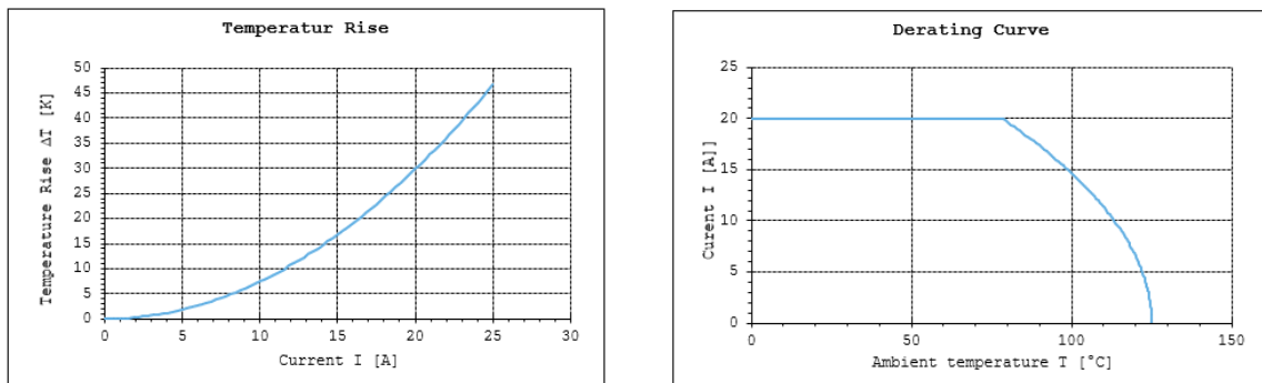
Figure 6. Current &amp; Temperature-rise Curve, and Derating Curve of TE UPM HC 4P power
