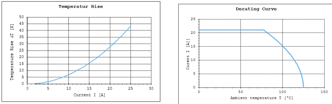
Figure 5. Current &amp; Temperature-rise Curve, and Derating Curve of TE UPM HC 3P power
