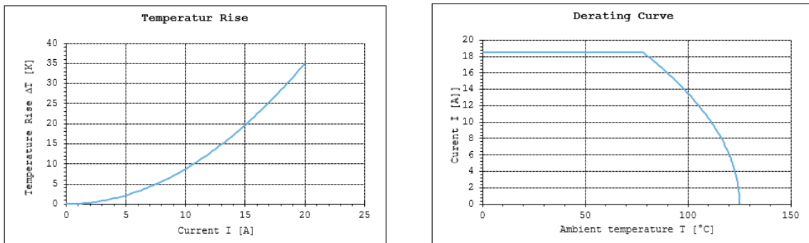
Figure 7. Current &amp; Temperature-rise Curve, and Derating Curve of TE UPM HC 8P power
