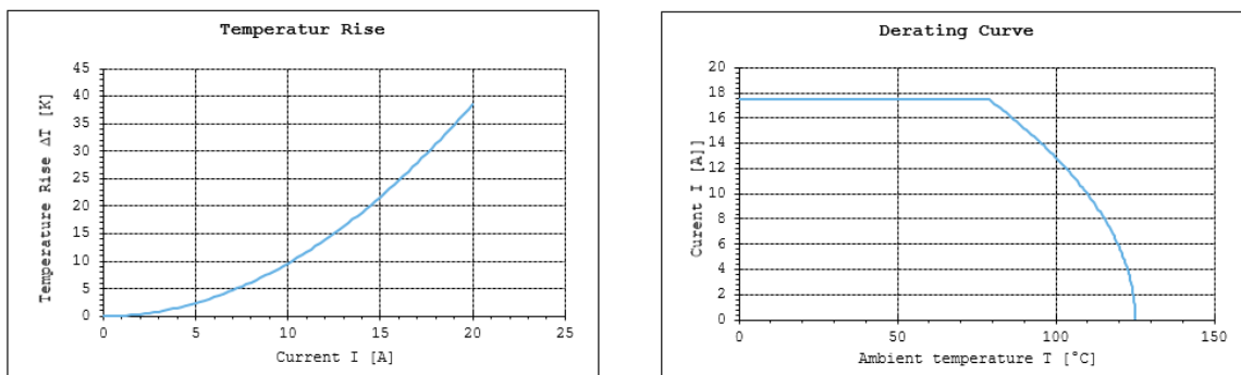
Figure 8. Current &amp; Temperature-rise Curve, and Derating Curve of TE UPM HC 12P power
