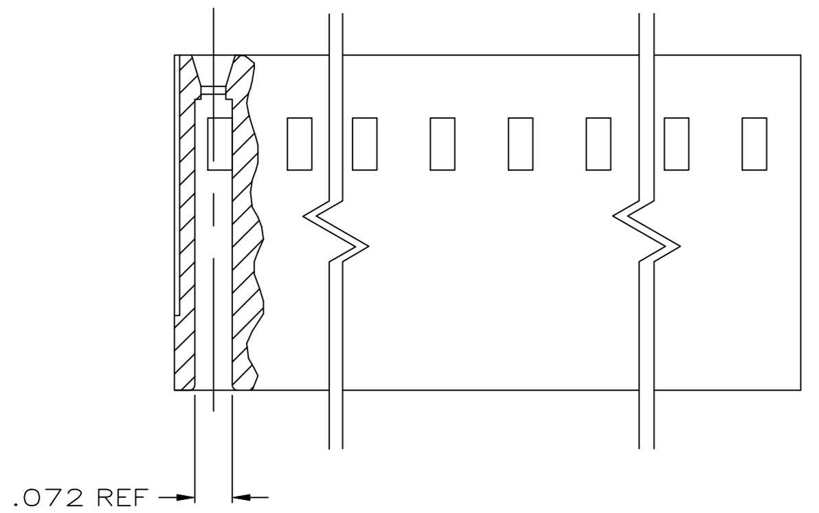
SECT X-X
