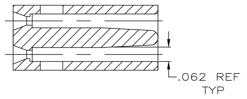
SECT Y-Y
