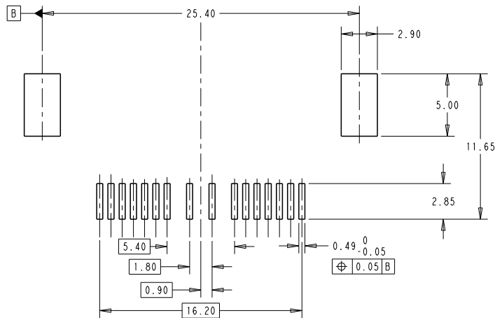
RECOMMEND PCB LAYOUT TOLERANCE: ±0.05mm
