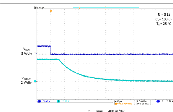
Figure 7-37. Turnoff Delay and Fall Time With 100-μF Load
