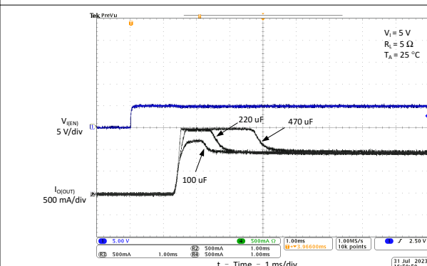
Figure 7-39. Inrush Current With Different Load Capacitance
