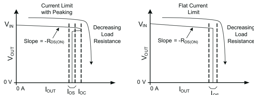
Figure 9-4. Current Limit Profiles
