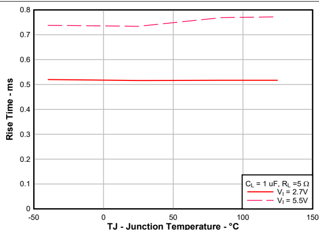
Figure 7-26. Rise Time vs Input Voltage
