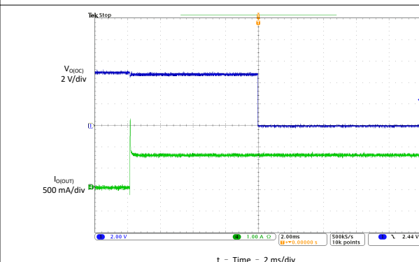
Figure 7-41. 2-Ω Load Connected to Enabled Device
