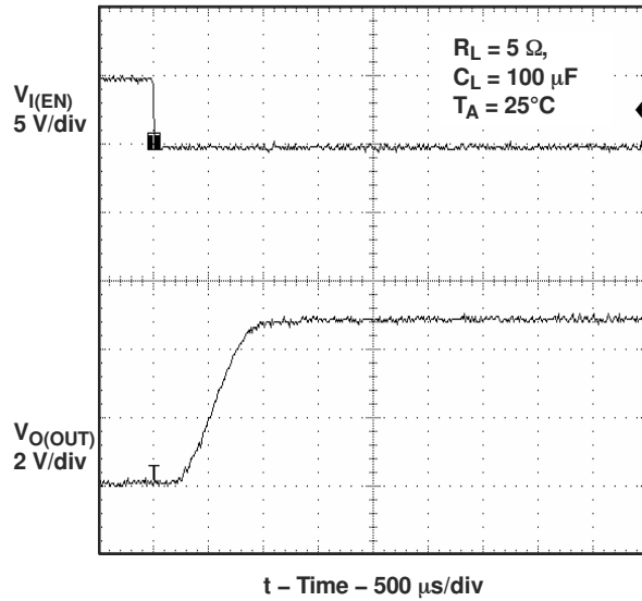
Figure 7-18. Turnon Delay and Rise Time With 100- \mu F Load
