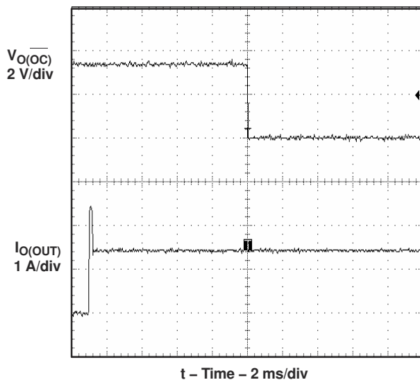
Figure 7-22. 2- \Omega Load Connected to Enabled Device
