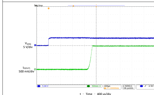
Figure 7-38. Short-Circuit Current, Device Enabled Into Short
