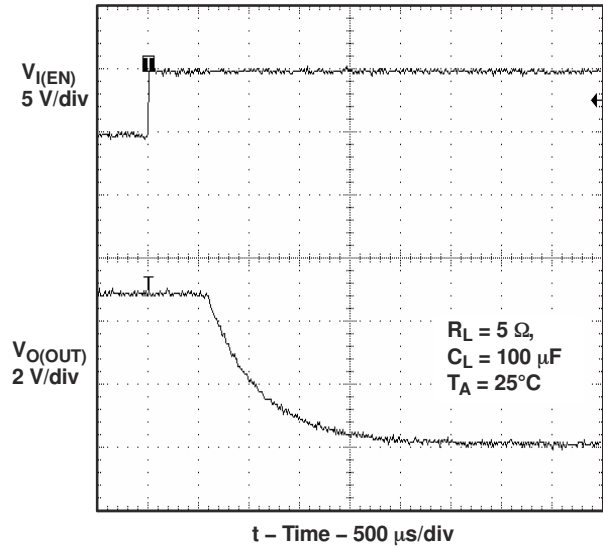
Figure 7-19. Turnoff Delay and Fall Time With 100- \mu F Load
