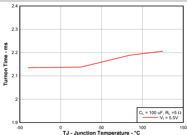
Figure 7-24. Turnon Time vs Junction Temperature
