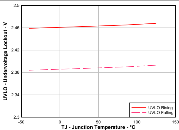
Figure 7-32. Undervoltage Lockout vs Junction Temperature
