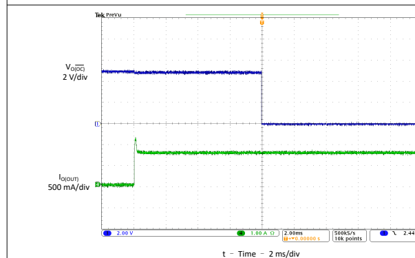
Figure 7-40. 3-Ω Load Connected to Enabled Device
