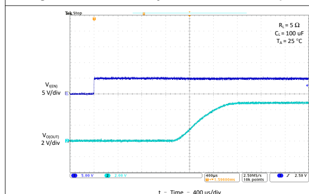
Figure 7-36. Turnon Delay and Rise Time With 100-μF Load
