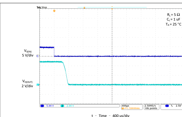
Figure 7-35. Turnoff Delay and Fall Time With 1-μF Load
