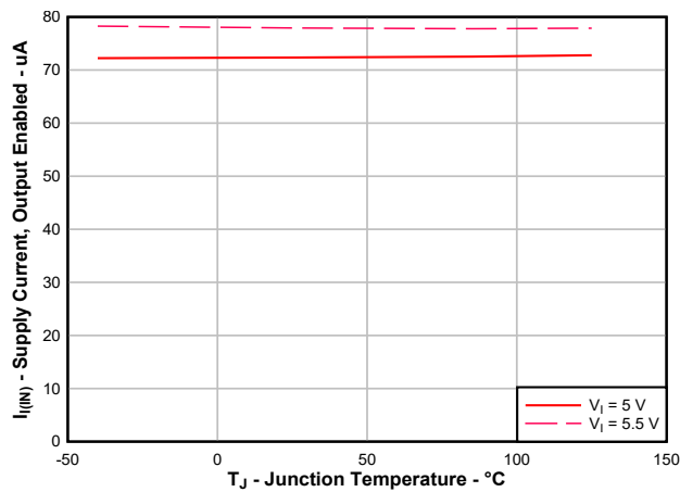
Figure 7-28. TPS2065DBV Supply Current, Output Enabled vs Junction Temperature
