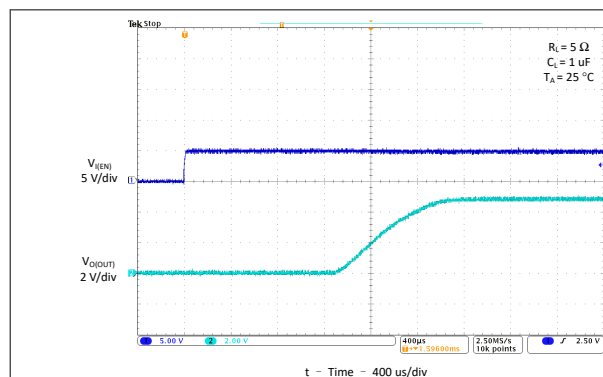
Figure 7-34. Turnon Delay and Rise Time With 1-μF Load
