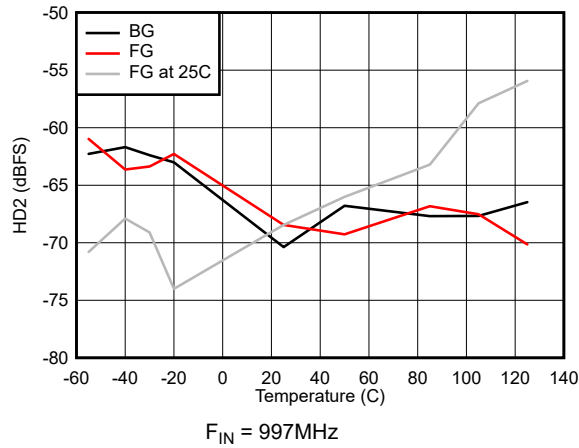
Figure 7-37. HD2 vs Temperature
