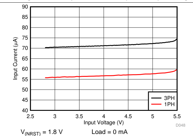
Figure 5. PFM Mode Current Consumption vs Input Voltage, One Regulator Enabled (3+1-Phase Output)
