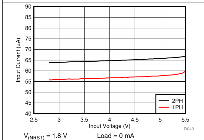
Figure 6. PFM Mode Current Consumption vs Input Voltage, One Regulator Enabled (2+1+1-Phase Output)
