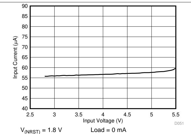
Figure 7. PFM Mode Current Consumption vs Input Voltage, One Regulator Enabled (1+1+1+1-Phase Output)
