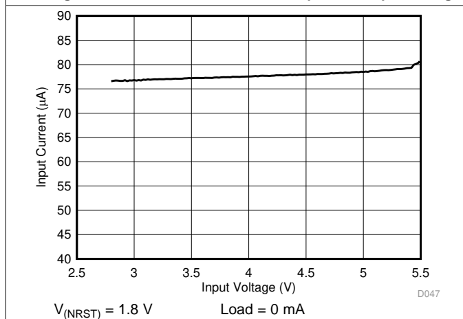
Figure 4. PFM Mode Current Consumption vs Input Voltage (4-Phase Output)
