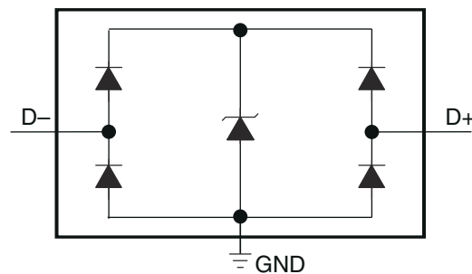
Figure 7-2. TPD2EUSB30/A Circuit
