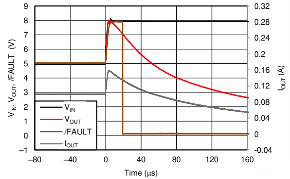
Figure 9-7. V_{IN} Step 5 V to 8 V with 4.7 \mu\text{F} // 100 \Omega
