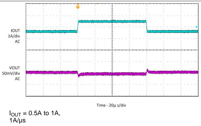
Figure 27. Load Transient
