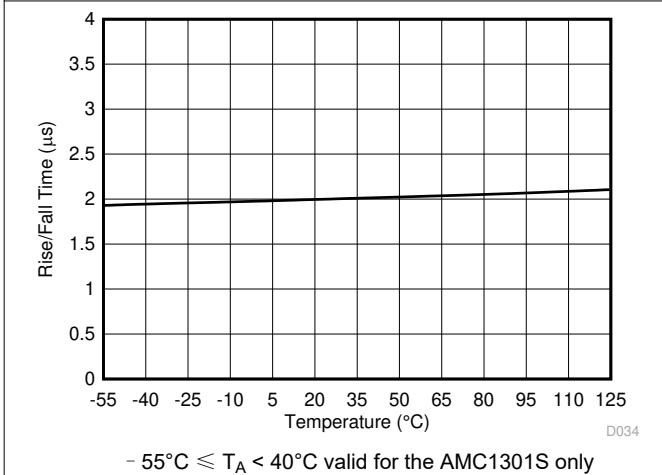
图 6-37. Output Rise and Fall Time vs Temperature
