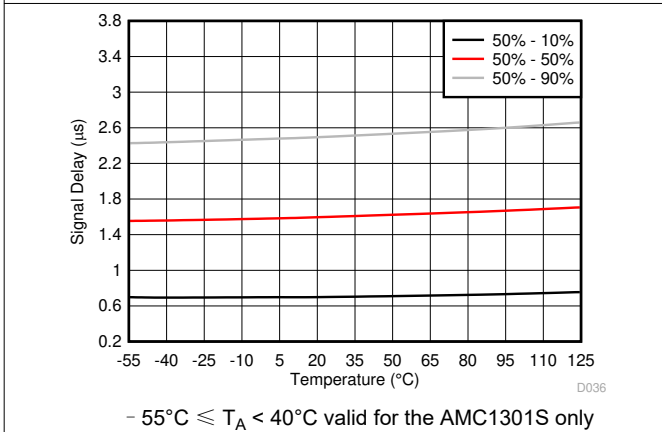
图 6-39. V_{IN} to V_{OUT} Signal Delay vs Temperature
