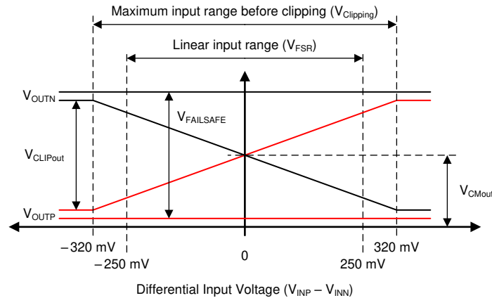
图 7-2. Output Behavior of the AMC1301
