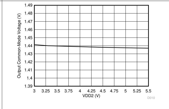
图 6-40. Output Common-Mode Voltage vs Low-Side Supply Voltage
