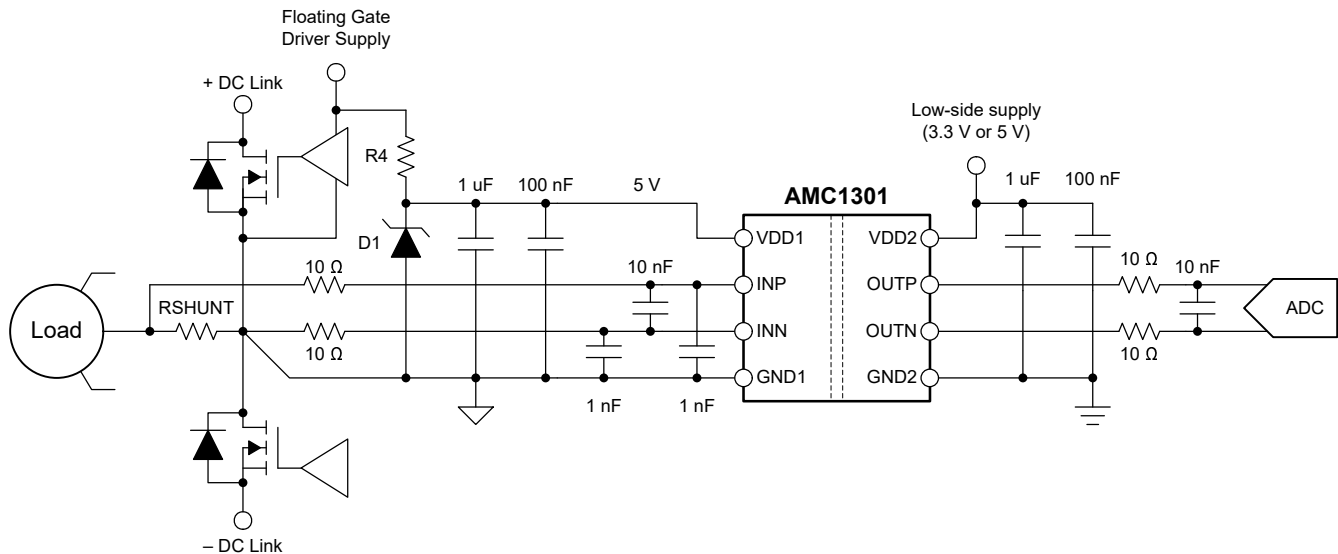
图 8-1. Using the AMC1301 for Current Sensing in a Typical Application
