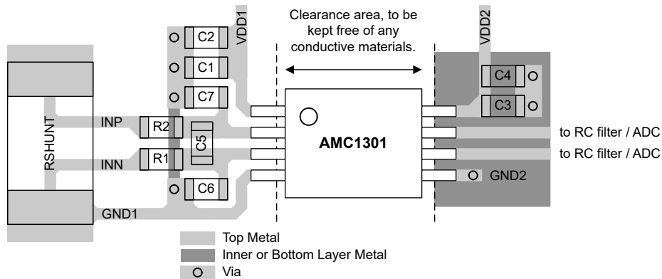
图 8-6. Recommended Layout of the AMC1301
