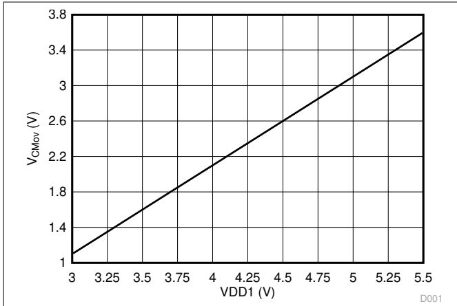
图 6-5. Common-Mode Overvoltage Detection Level vs High-Side Supply Voltage
