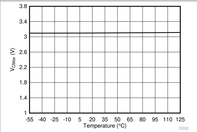
图 6-6. Common-Mode Overvoltage Detection Level vs Temperature
