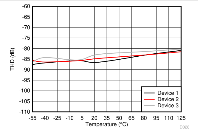
图 6-30. Total Harmonic Distortion vs Temperature
