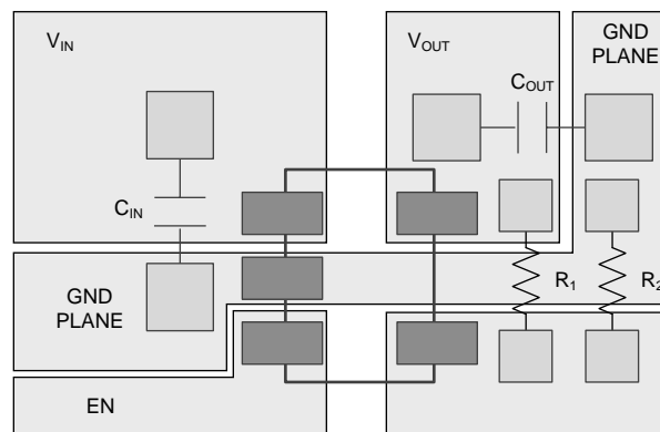
Figure 44. DBV Package Layout Example
