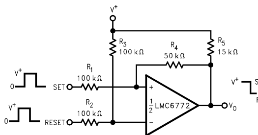
Figure 34. Bi-Stable Multivibrator
