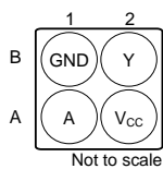
YFP Package 4-Pin DSBGA Bottom View
