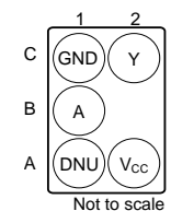
YZP Package 5-Pin DSBGA Bottom View
