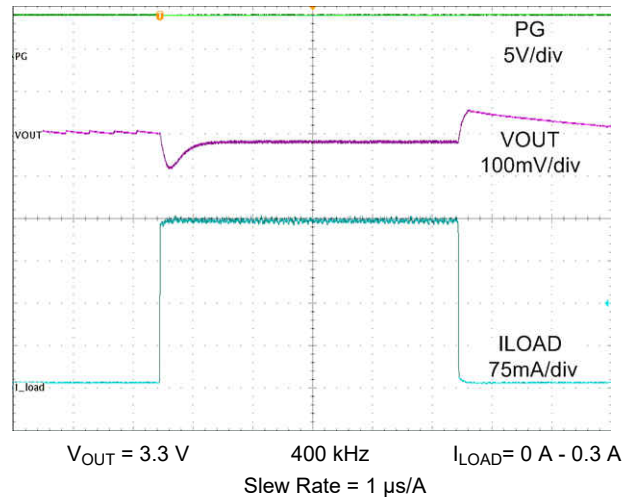
Figure 9-16. Load Transient
