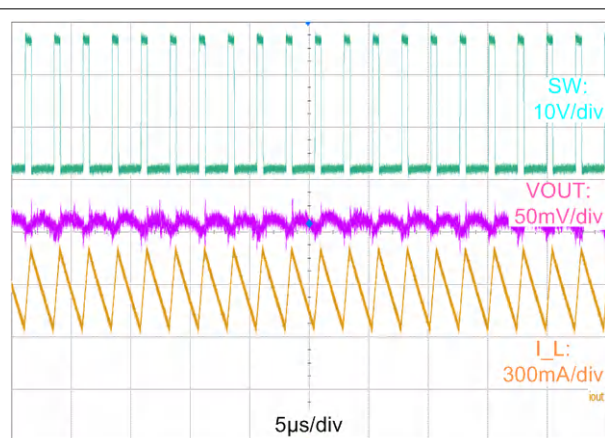
Figure 8-8. Typical PWM Switching Waveforms V_{IN} = 24\text{ V} , V_{OUT} = 5\text{ V} , I_{OUT} = 600\text{ mA} , f_s = 400\text{ kHz}
