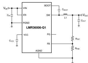
Simplified Schematic
