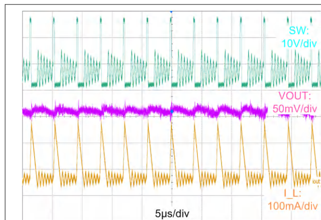
Figure 8-7. Typical PFM Switching Waveforms V_{IN} = 24\text{ V} , V_{OUT} = 5\text{ V} , I_{OUT} = 30\text{ mA}
