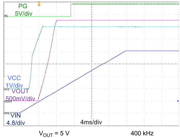
Figure 9-14. Start-Up Waveform
