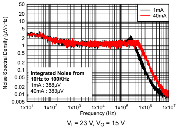
Figure 6-21. Noise Spectral Density vs Frequency and I_O for New Chip V_I = 23\text{ V} , V_O = 15\text{ V}
