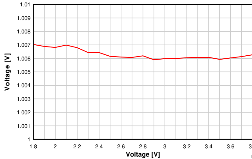
Figure 8-30. ADC Accuracy vs. Supply Voltage (VDD5)
