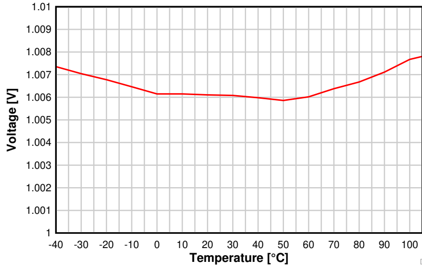
Figure 8-29. ADC Accuracy vs. Temperature
