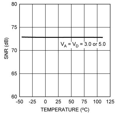
Figure 27. SNR vs. Temperature
