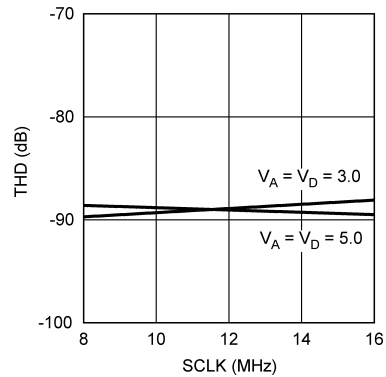
Figure 23. THD vs. SCLK
