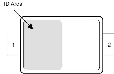
Figure 5-2. DYA Package 2-Pin SOD-523 Top View
