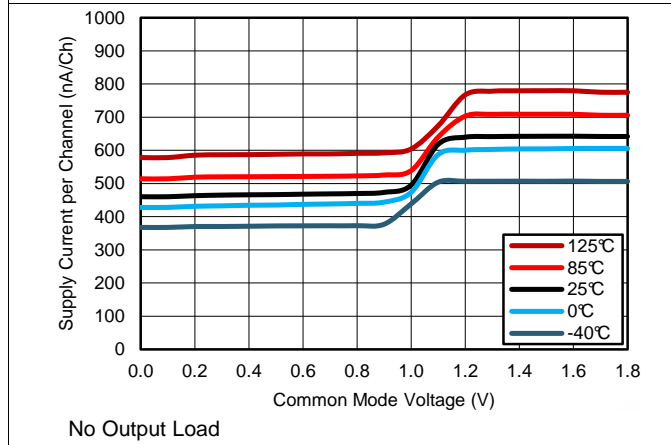
Figure 3. Supply Current vs Common Mode at 1.8 V
