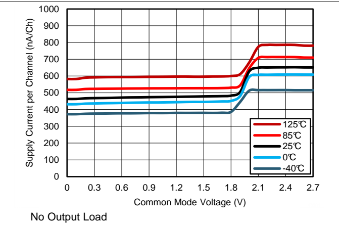
Figure 4. Supply Current vs Common Mode at 2.7 V
