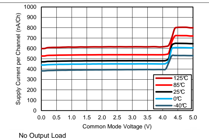
Figure 6. Supply Current vs Common Mode at 5 V
