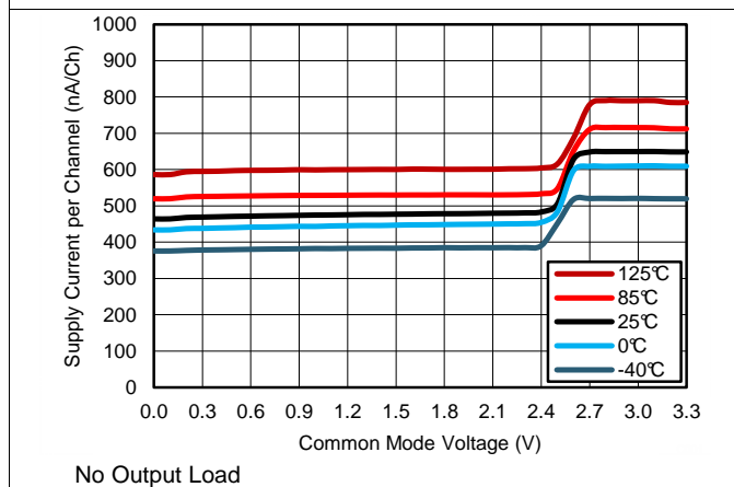
Figure 5. Supply Current vs Common Mode at 3.3 V
