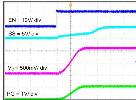
Figure 44. TPS563210A Start Up Relative To EN
