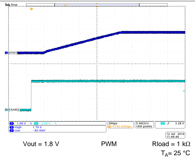
Figure 47. Start-Up Timing
