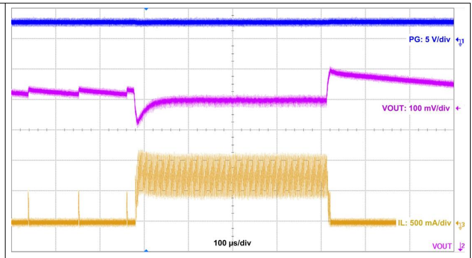
V_{OUT} = 3.3\text{ V} 400\text{ kHz} I_{LOAD} = 10\text{ mA} - 0.75\text{ A} Slew Rate = 1\text{ }\mu\text{s/A}
