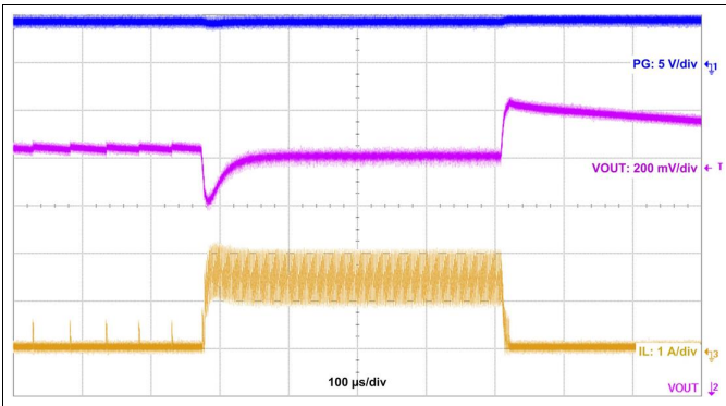
V_{OUT} = 5\text{ V} 400\text{ kHz} I_{LOAD} = 10\text{ mA} - 0.75\text{ A} Slew Rate = 1\text{ }\mu\text{s/A}
