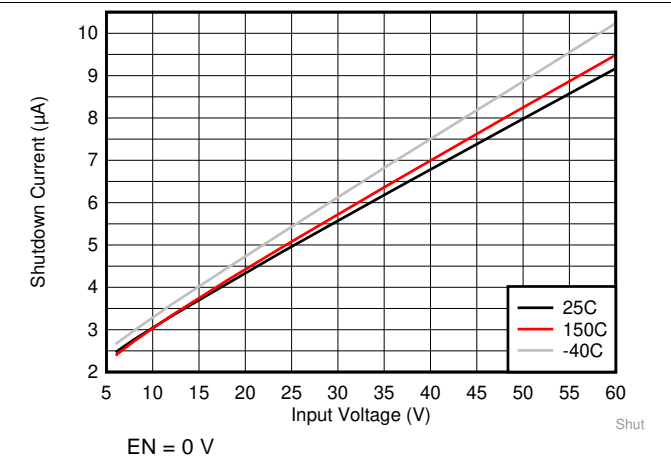
图 2. Shutdown Supply Current
