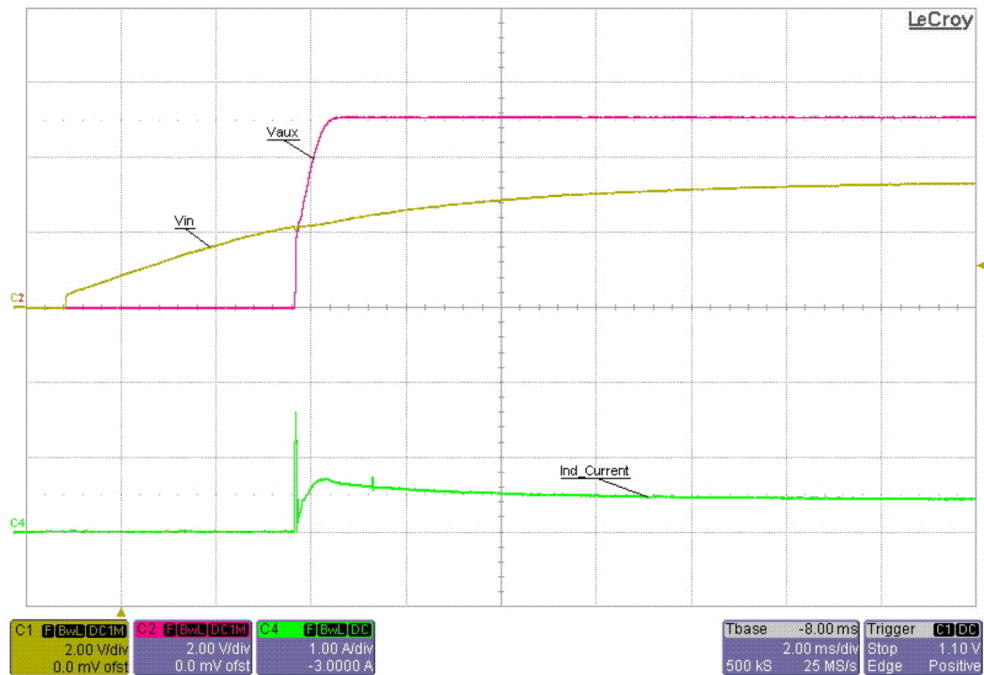
Figure 33. Start-Up, V_{IN} = 3.3\text{ V} , I_{AUX} = 0.5\text{ A} , USB Switch Disabled
