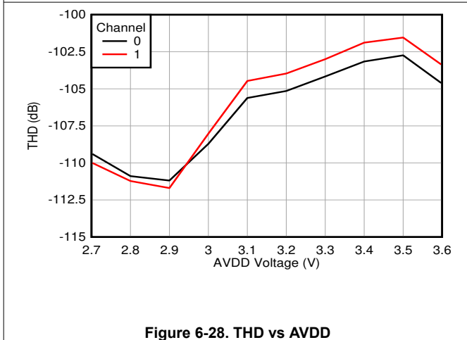
Figure 6-28. THD vs AVDD
