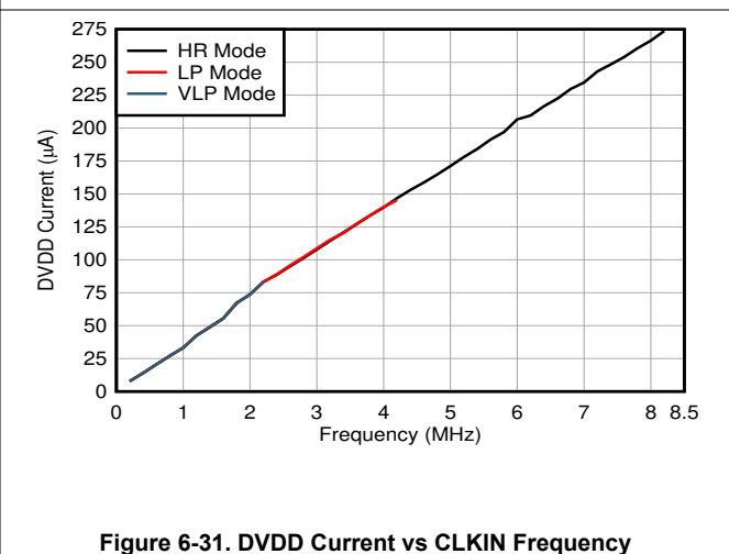
Figure 6-31. DVDD Current vs CLKIN Frequency
