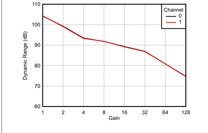
Figure 6-24. Dynamic Range vs Gain
