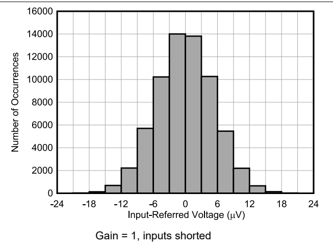
Figure 6-21. Single Device Noise Histogram at 32 kSPS
