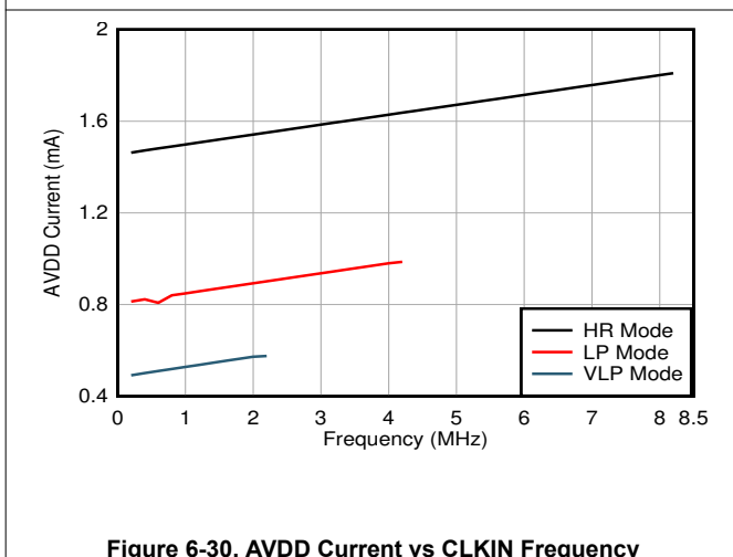
Figure 6-30. AVDD Current vs CLKIN Frequency
