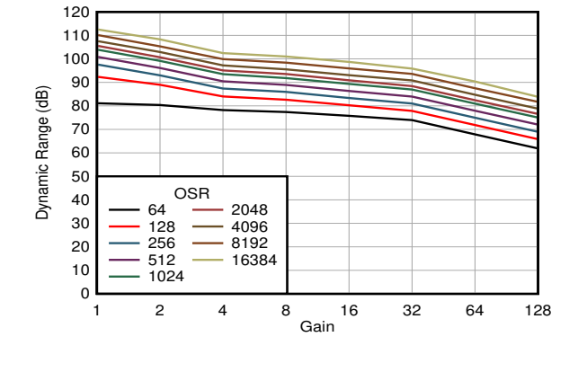
Figure 6-25. Dynamic Range vs Gain
