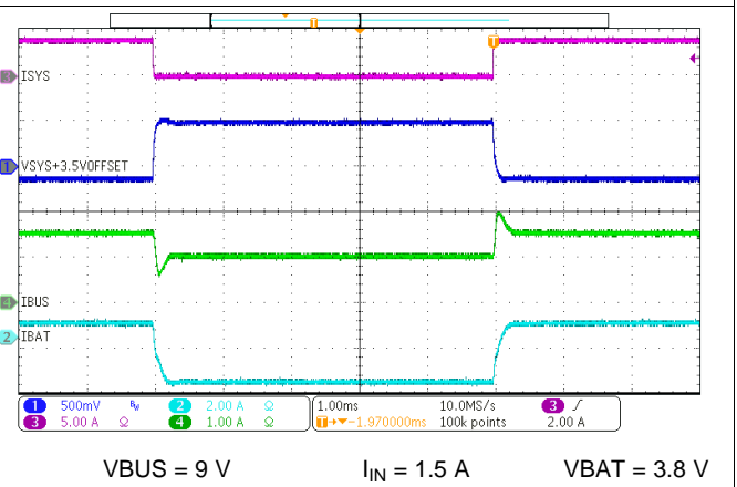
Figure 53. Charge Disable
