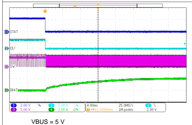
Figure 52. Charge Enable
