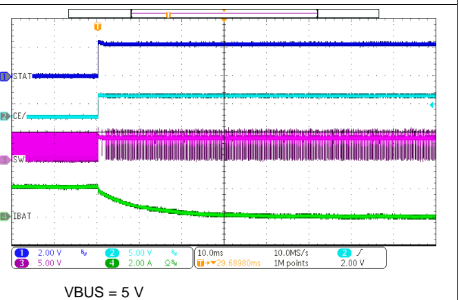
Figure 53. Charge Disable
