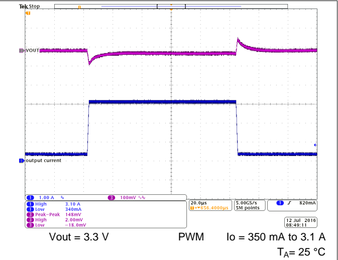
Figure 51. Load Transient Response
