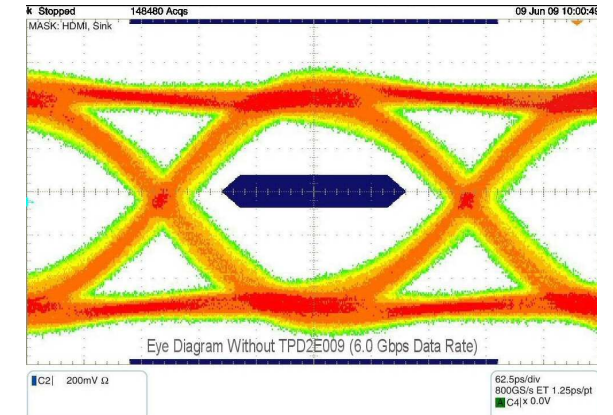
Figure 13. Eye Diagram Without TPD2E009 (6-Gbps Data Rate) (3-Pin DBZ Package)
