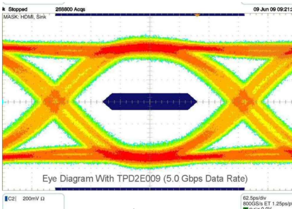
Figure 10. Eye Diagram With TPD2E009 (5-Gbps Data Rate) (3-Pin DBZ Package)
