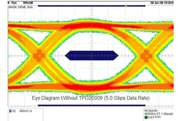
Figure 11. Eye Diagram Without TPD2E009 (5-Gbps Data Rate) (3-Pin DBZ Package)
