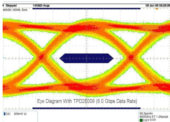
Figure 12. Eye Diagram With TPD2E009 (6-Gbps Data Rate) (3-Pin DBZ Package)
