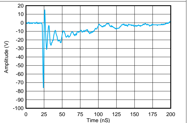
Figure 6. IEC Clamping Waveforms (-8-kV Contact)
