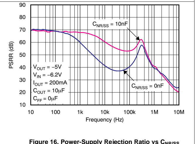
Figure 16. Power-Supply Rejection Ratio vs C_{NR/SS}
