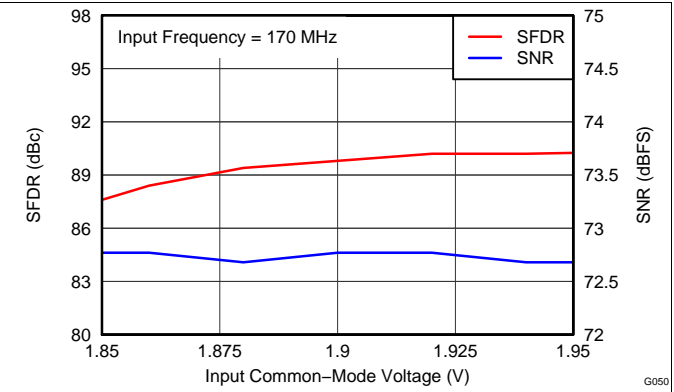
Figure 50. Performance vs Input Common-Mode Voltage (170 MHz)
