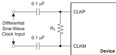
Figure 117. Differential Sine-Wave Clock Driving Circuit
