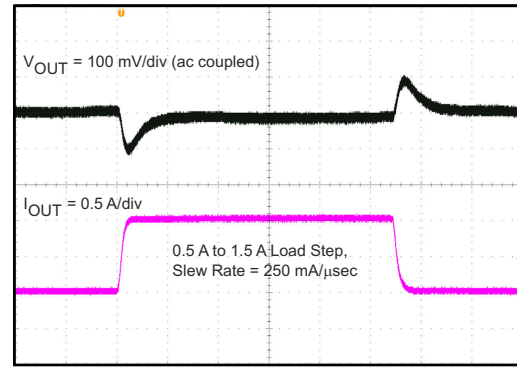
Time - 200 \mu s/div 0.5 至 1.5A
