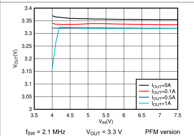
Figure 7-6. 3.3-V Dropout
