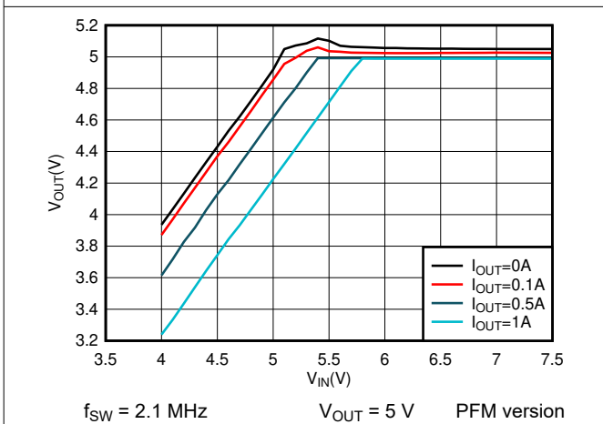
Figure 7-5. 5-V Dropout
