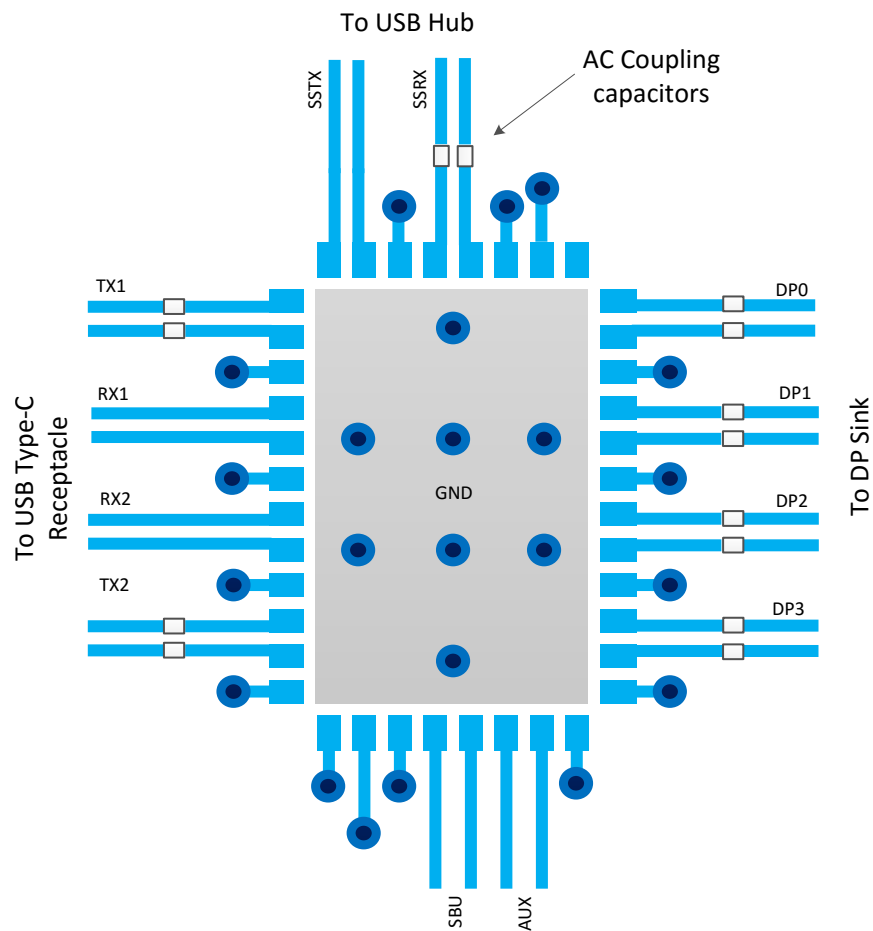
Figure 11-1. Layout Example
