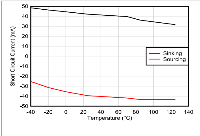
Figure 5-31. Short-Circuit Current vs Temperature
