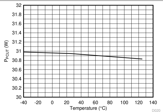
图 7-20. P_Cut Threshold (30W) vs Temperature
