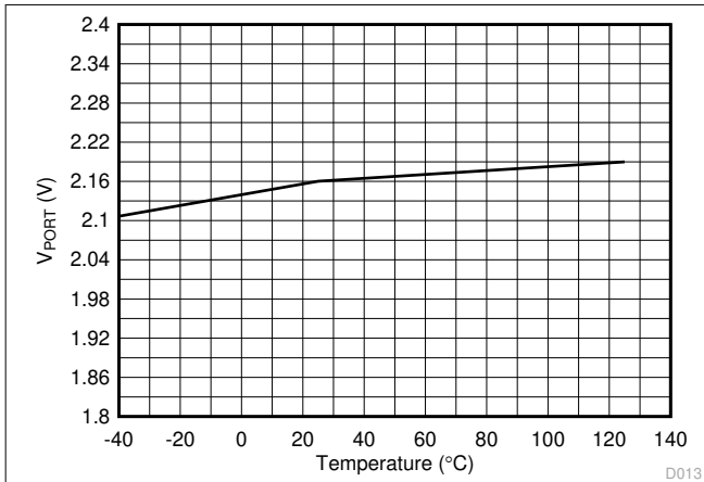
图 7-13. Power Good Threshold vs Temperature
