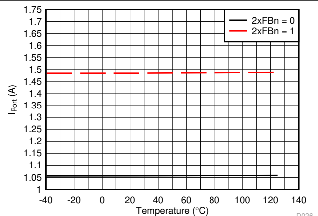
图 7-24. I_SHORT Threshold vs Temperature
