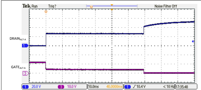
图 10-3. I_{LIM} Foldback and Turn-Off
