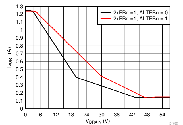
图 7-28. 2x Mode (2xFBn = 1) Current Foldback vs Drain Voltage
