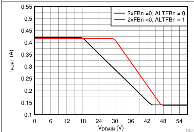
图 7-27. 1x Mode (2xFBn = 0) Current Foldback vs Drain Voltage
