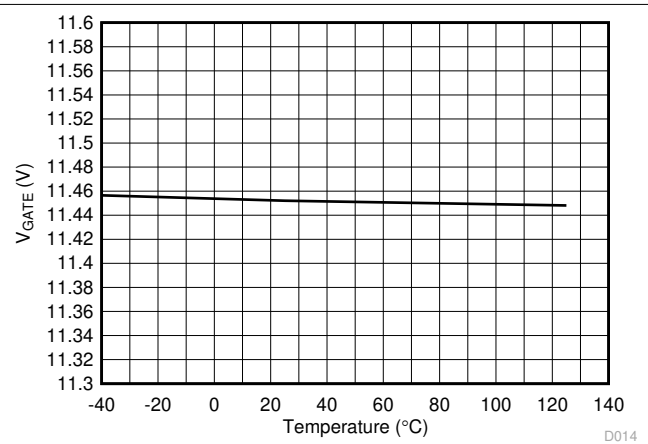
图 7-14. Gate Voltage (Port On) vs Temperature
