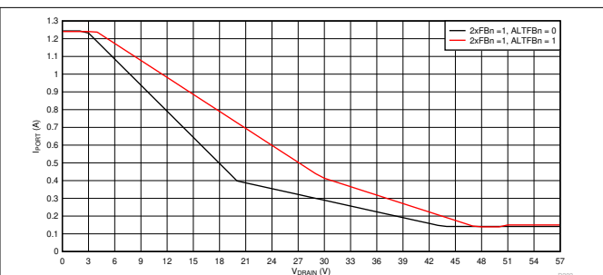
图 9-52. 2x Mode (2xFBn = 1) Foldback Curves, I_{PORT} vs V_{DRAIN}
