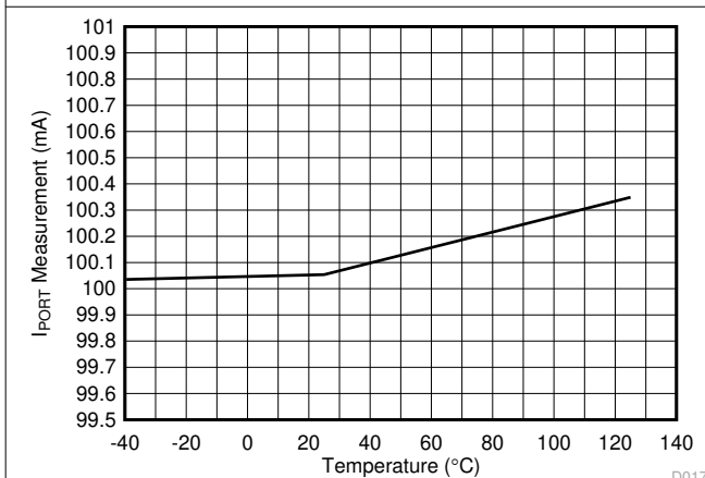
图 7-17. Port Current ADC Measurement (100mA) vs Temperature
