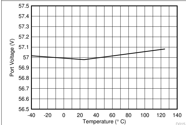
图 7-15. Port Voltage ADC Measurement vs Temperature
