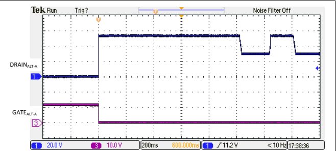
图 10-4. Backoff Due to PCut Fault
