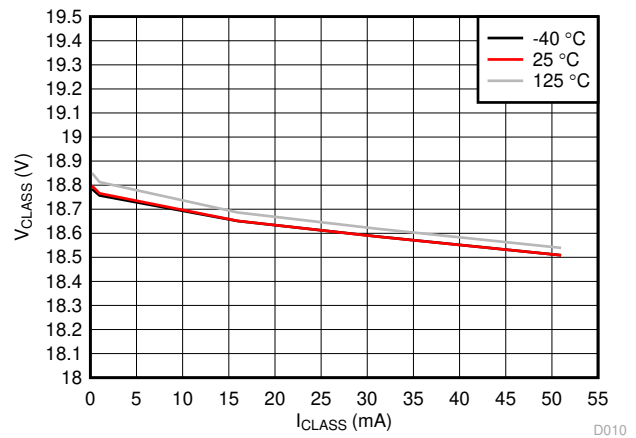
图 7-10. Classification Voltage vs I_{CLASS} and Temperature
