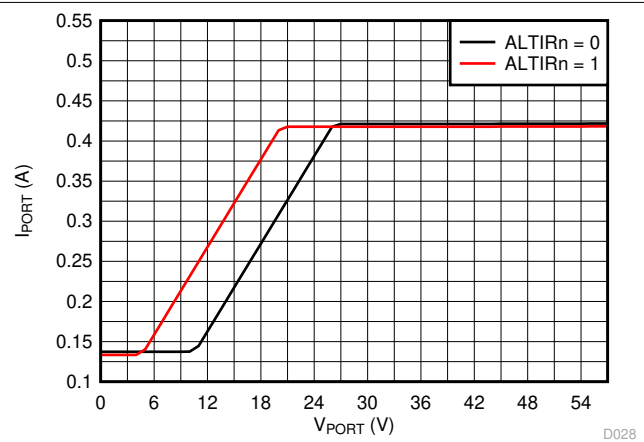
图 7-26. Inrush Current Foldback vs Port Voltage
