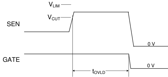
图 8-2. Overcurrent Fault Timing
