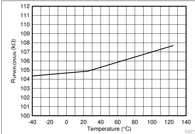
图 7-25. R OFF (VPWR to DRAIN) vs Temperature
