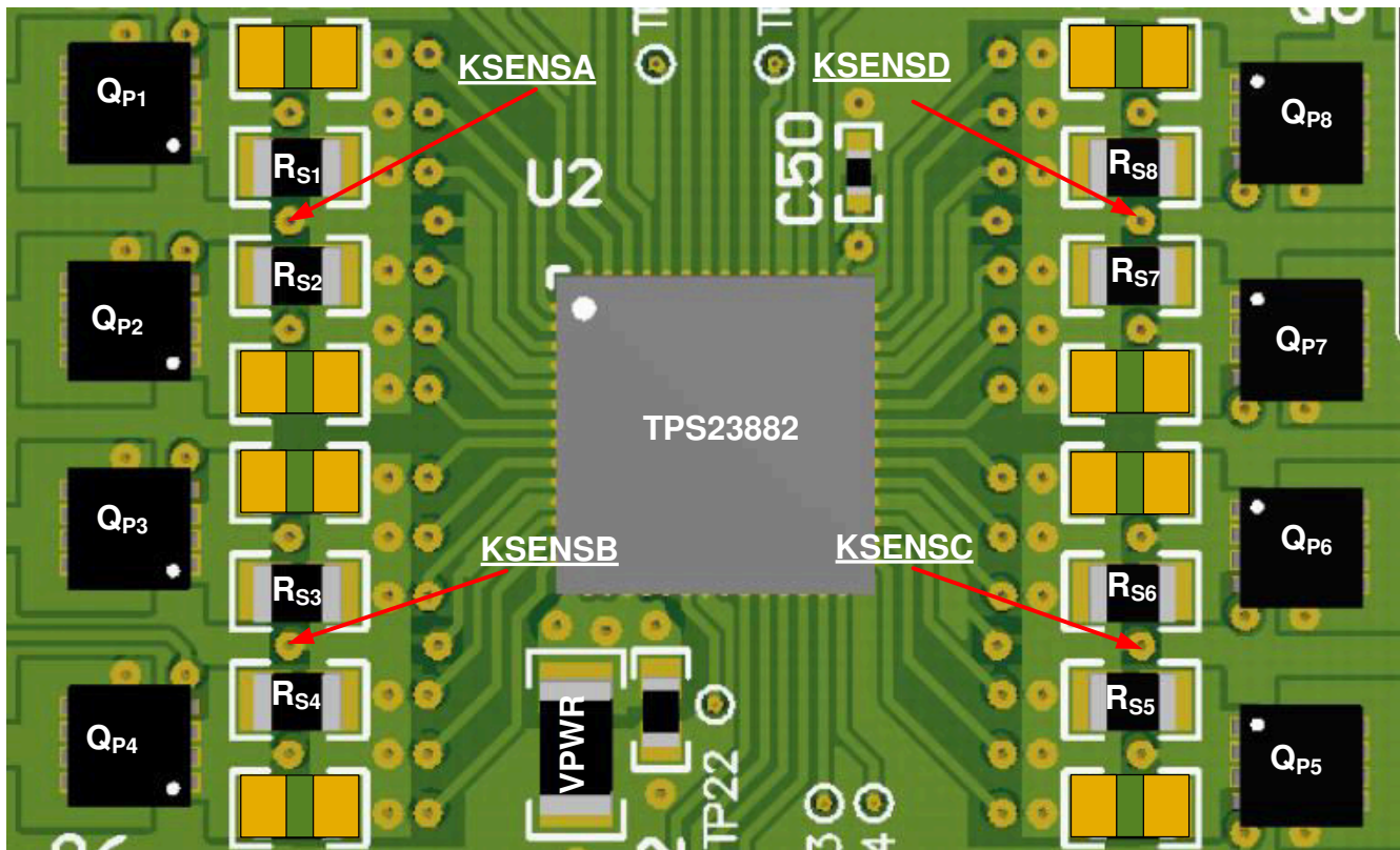
图 12-3. Eight Port Layout Example (Top Side)
