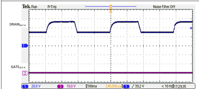
图 10-5. Open Circuit Detection Signature
