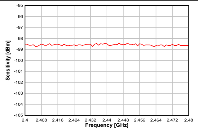
图 8-11. Sensitivity vs. Frequency (IEEE 802.15.4-2006, 250 kbps, OQPSK DSSS 1:8, 2.44 GHz)
