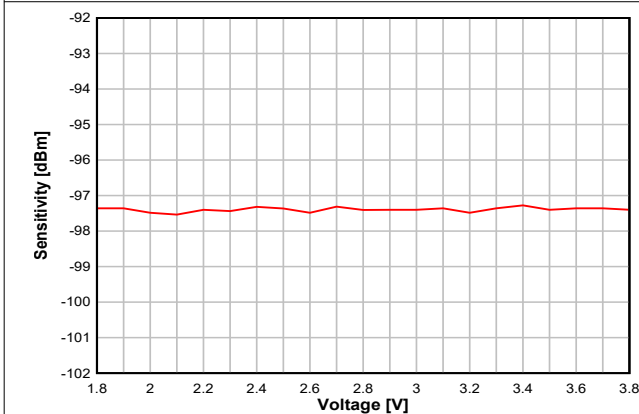
图 8-14. Sensitivity vs. Supply Voltage (VDD5) (BLE 1 Mbps, 2.44 GHz)
