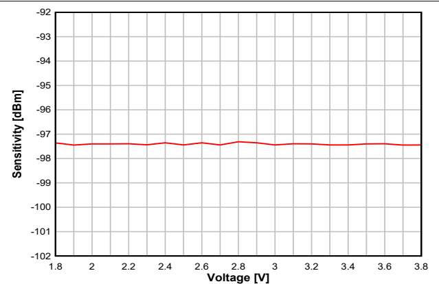
图 8-15. Sensitivity vs. Supply Voltage (VDD5) (BLE 1 Mbps, 2.44 GHz, DCDC Off)
