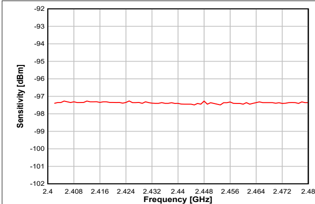
图 8-10. Sensitivity vs. Frequency (BLE 1 Mbps, 2.44 GHz)
