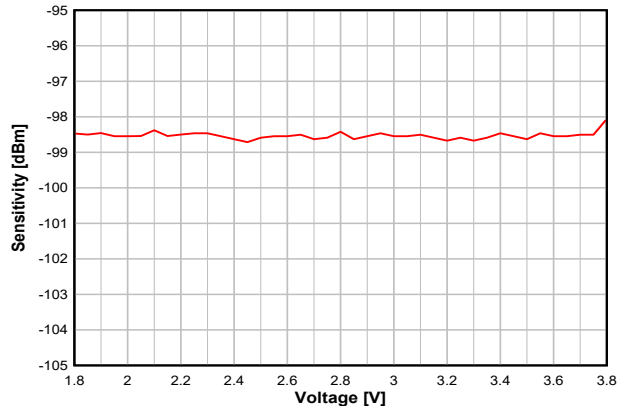
图 8-16. Sensitivity vs. Supply Voltage (VDDS) (IEEE 802.15.4-2006, 250 kbps, OQPSK DSSS 1:8, 2.44 GHz)
