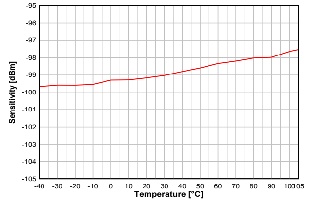
图 8-13. Sensitivity vs. Temperature (IEEE 802.15.4-2006, 250 kbps, OQPSK DSSS 1:8, 2.44 GHz)
