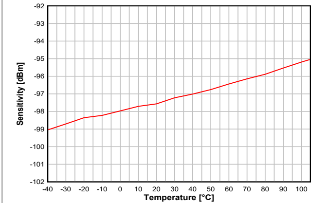
图 8-12. Sensitivity vs. Temperature (BLE 1 Mbps, 2.44 GHz)
